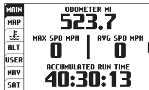
Main Tab 2
