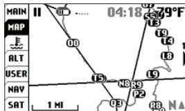
Map Screen 1
